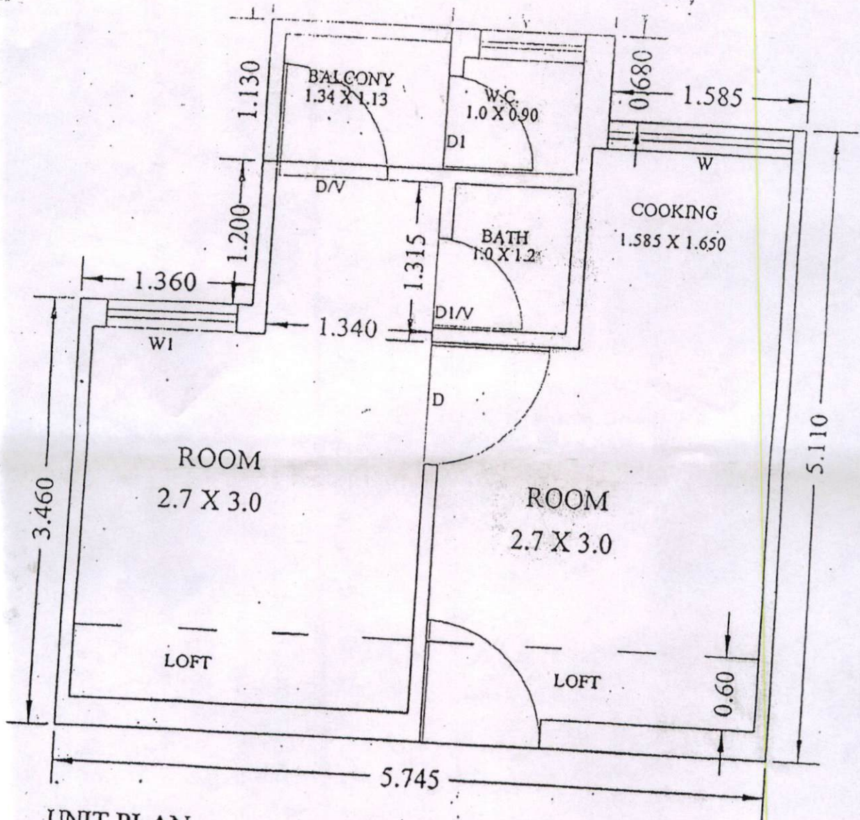
UNIT PLAN
